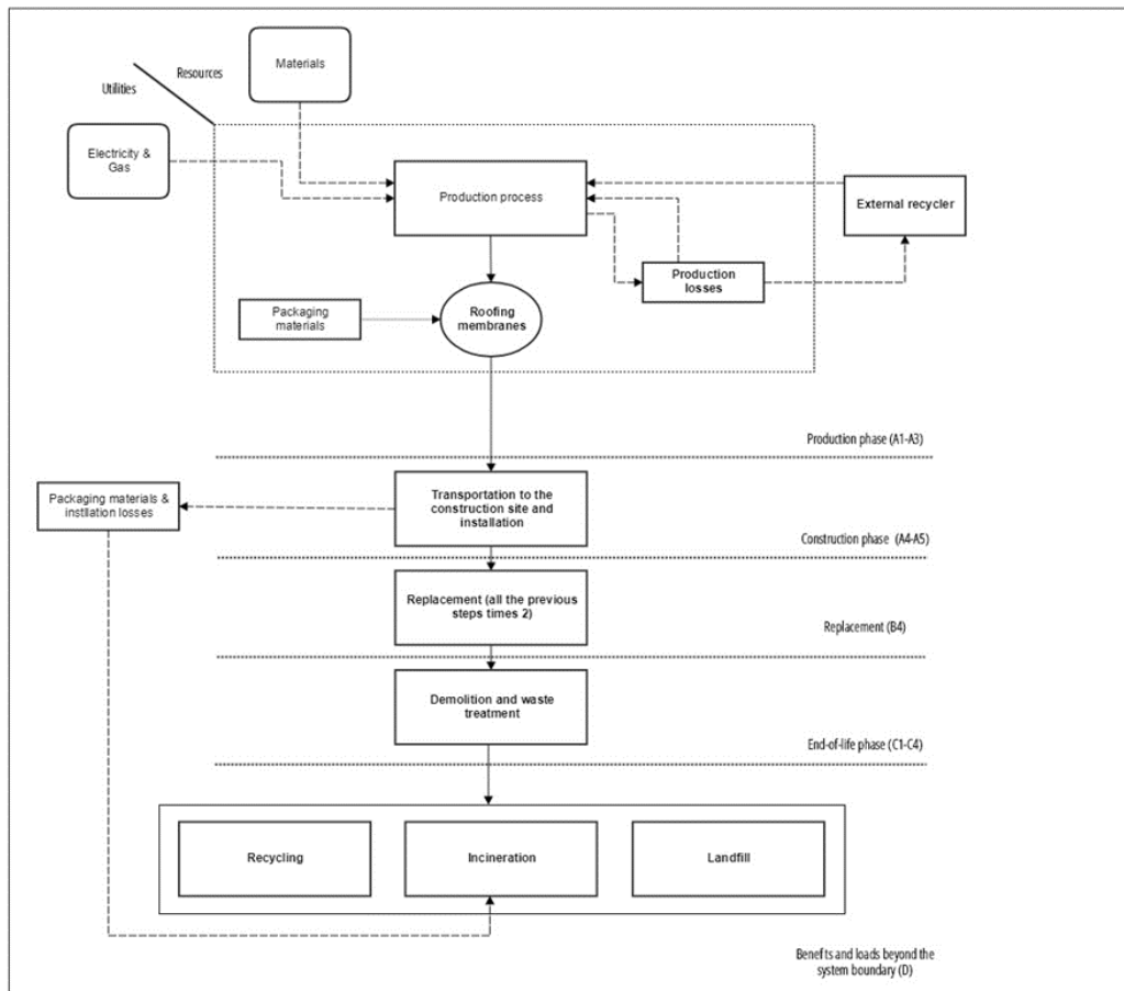
Figure 1: Process tree of one m² of Alkotec A SK.
